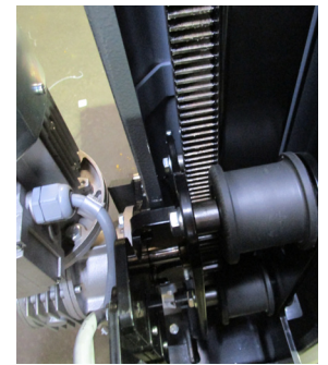
Rack & Pinion carriage drive system for added reliability
